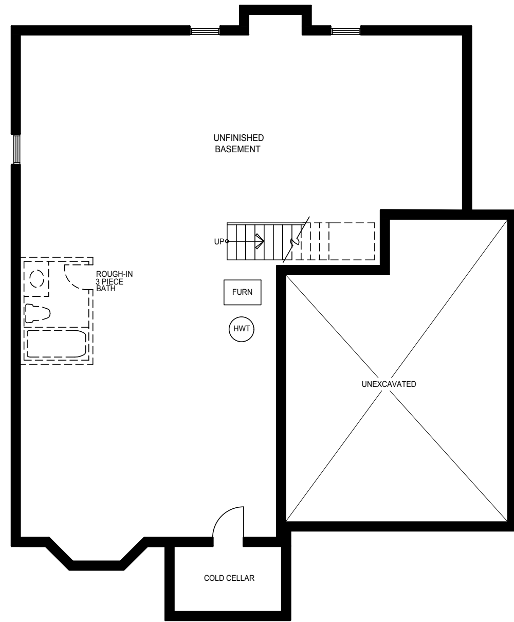
BASEMENT PLAN ELEVATION 'B'
