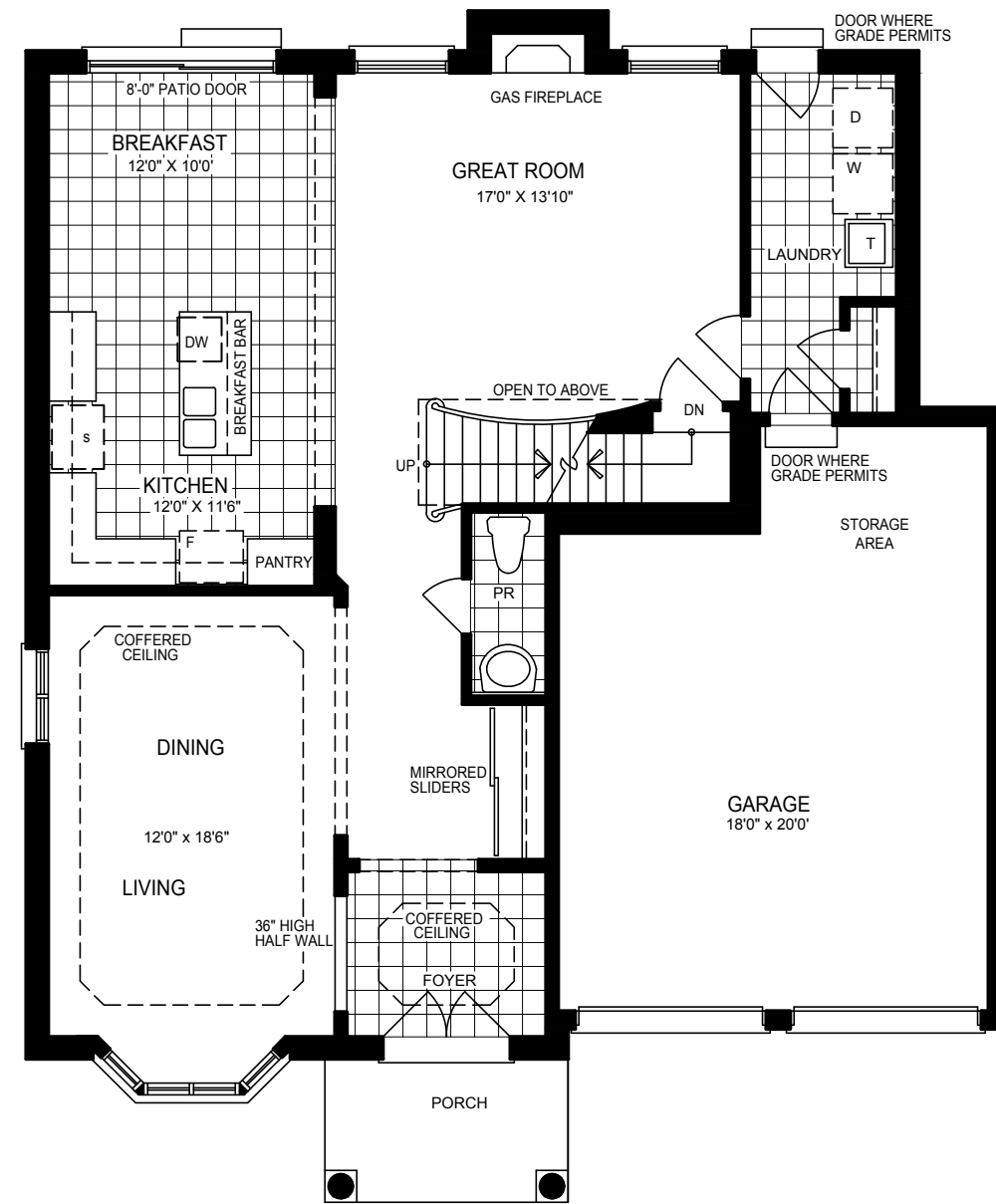
GROUND FLOOR PLAN ELEVATION 'B'
