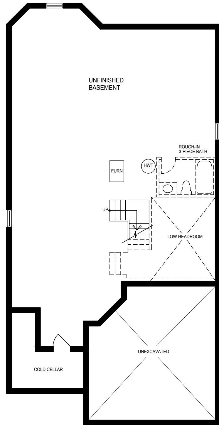
BASEMENT PLAN ELEVATION 'C'
