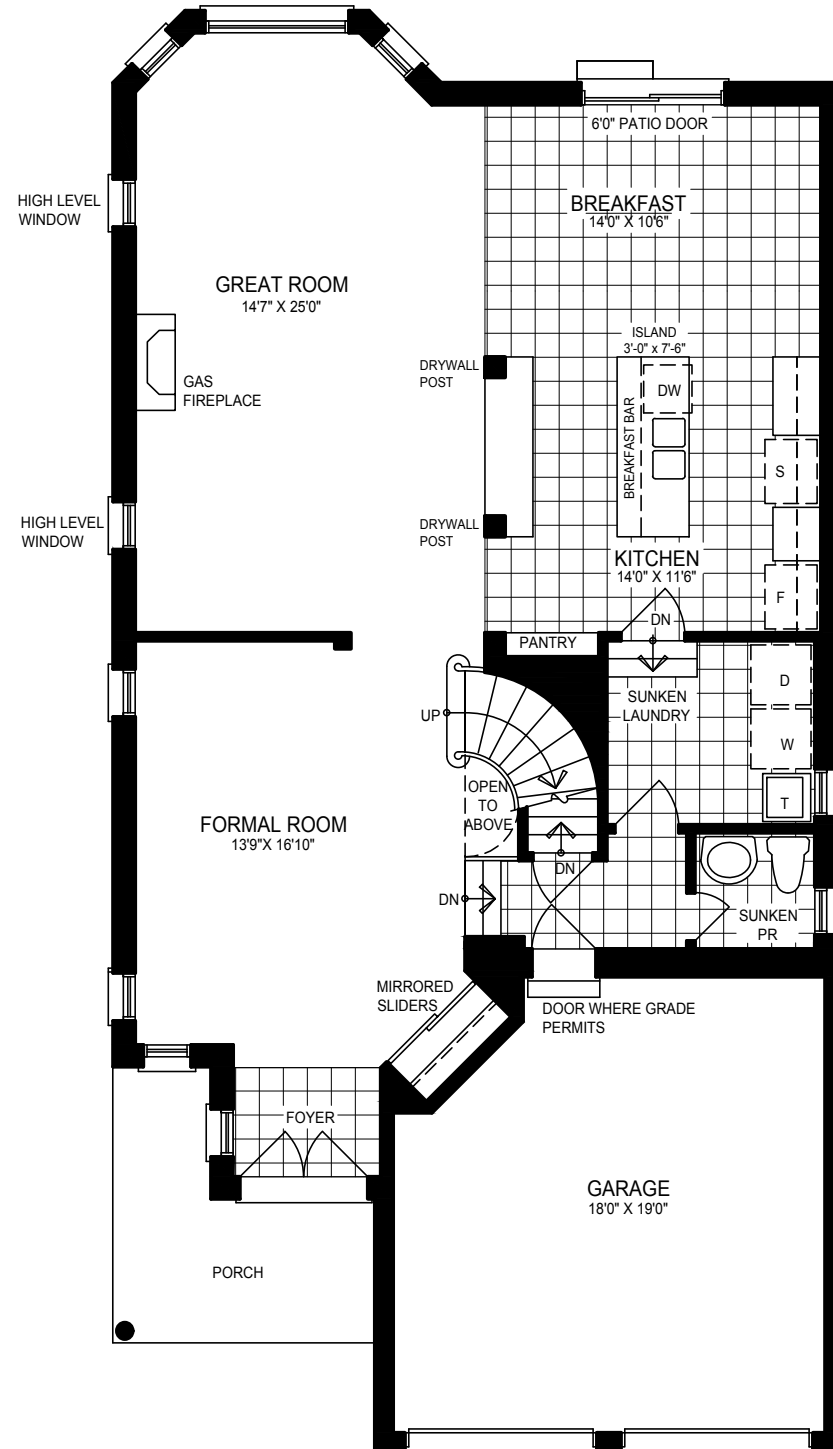
GROUND FLOOR PLAN ELEVATION 'C'
